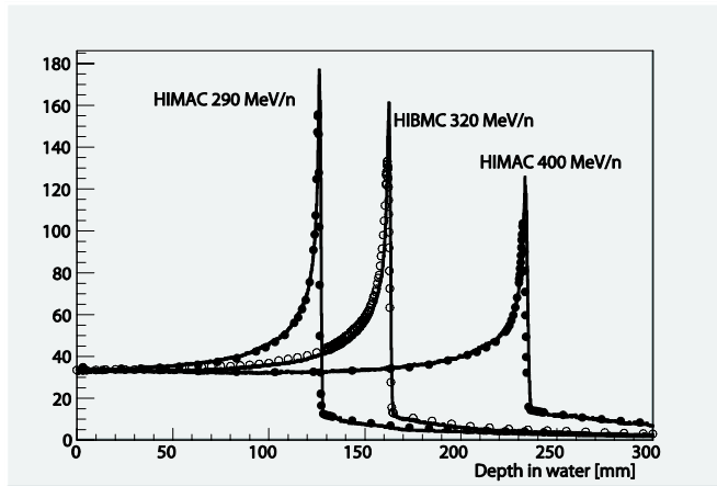
Fig. 3 Simulated depth-dose curves along with published data 10) for HIMAC 290 and 400 MeV/u and new data for HIBMC beam
