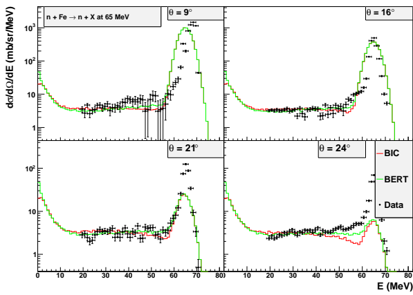
Fig. 6 n+Fe @ 65 MeV, neutron production
