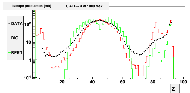
Fig. 4 p+U @ 1 GeV/A (inverse kinematics) residue production
