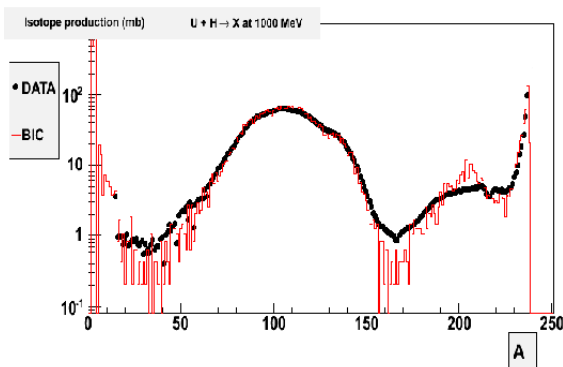
Fig. 13 Improved: p+U @ 1 GeV/A (inverse kinematics) residue production. Same comments as in previous figure apply here
