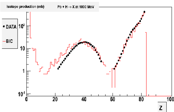
Fig. 12 Improved: p+Pb @ 1 GeV/A (inverse kinematics) residue production. Deep spallation region ( shoulder at the right side of the plot) can be better reproduced after ad hoc parameter tuning
