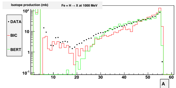
Fig. 2 p+Fe @ 1 GeV, residue production
