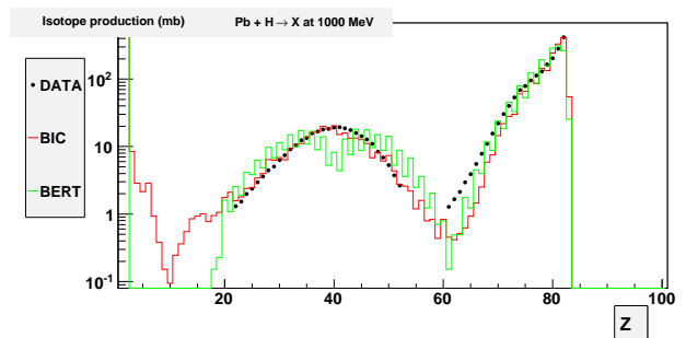
Fig. 3 p+Pb @ 1 GeV/A (inverse kinematics) residue production
