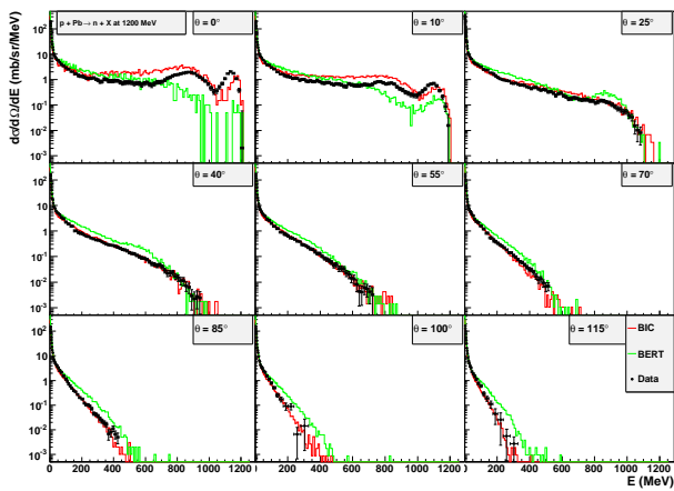
Fig. 7 p+Pb @ 1200 MeV, neutron production
