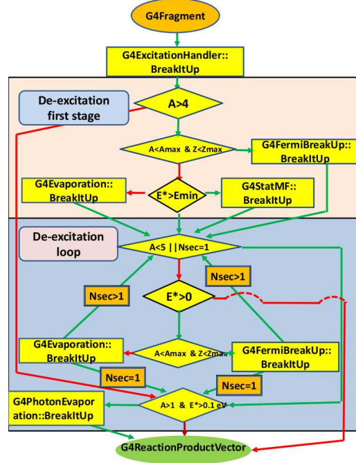
Fig. 1 Basic de-excitation diagram in v9.3. Nsec stands for the number of secondaries
