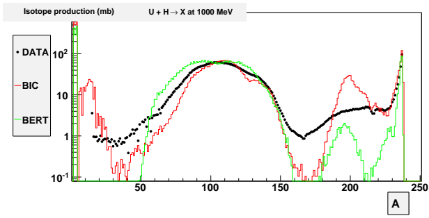
Fig. 5 p+U @ 1 GeV/A (inverse kinematics) residue production
