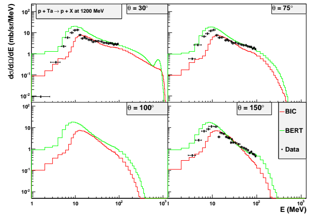
Fig. 8 p+Ta @ 1.2 GeV, proton production
