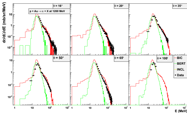
Fig. 11 p+Au @ 1.2 GeV, ^4\text{He} production
