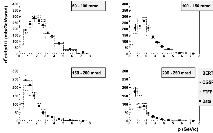
Figure 1. Double differential cross sections of \pi^+ forward production by 12 GeV/c protons off thin Carbon target: histograms – Geant4 9.3p01 simulation (BERT, QGSP, FTFP), points are data (Catanesi et al. 2008).
