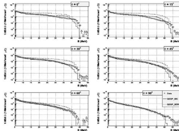
Figure 2. Double differential neutron yield measured from 50 MeV proton beam absorbed in the thick aluminum target: histograms – Geant4 9.3p01 simulations (QGSP_BIC and QGSP_BERT), points - data (Aoki et al. 2004).
