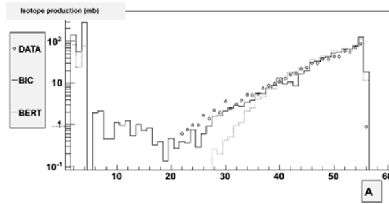
Figure 3. Isotope production cross section in inverse kinematic reaction of 500 MeV/u Fe ion in the Hydrogen target: histograms - Geant4 9.3p01 simulation (BIC and BERT), points are data (Villagrasa et al. 2005).
